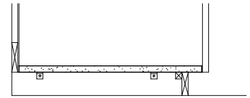
153a Section Detail of Removable Base / Toe Supported on Clips
